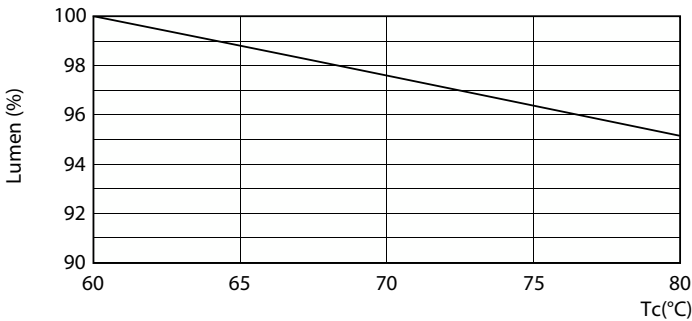
Lumen Maintenance Diagram - Ledtube DE 600mm 9W 900lm 740 T8 G13
