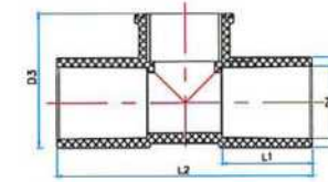
Faucet Tee 90° (With Brass Thread)
