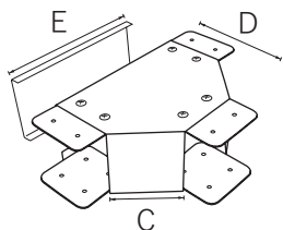
Top opening-Type 1 頂開蓋型-款式1
